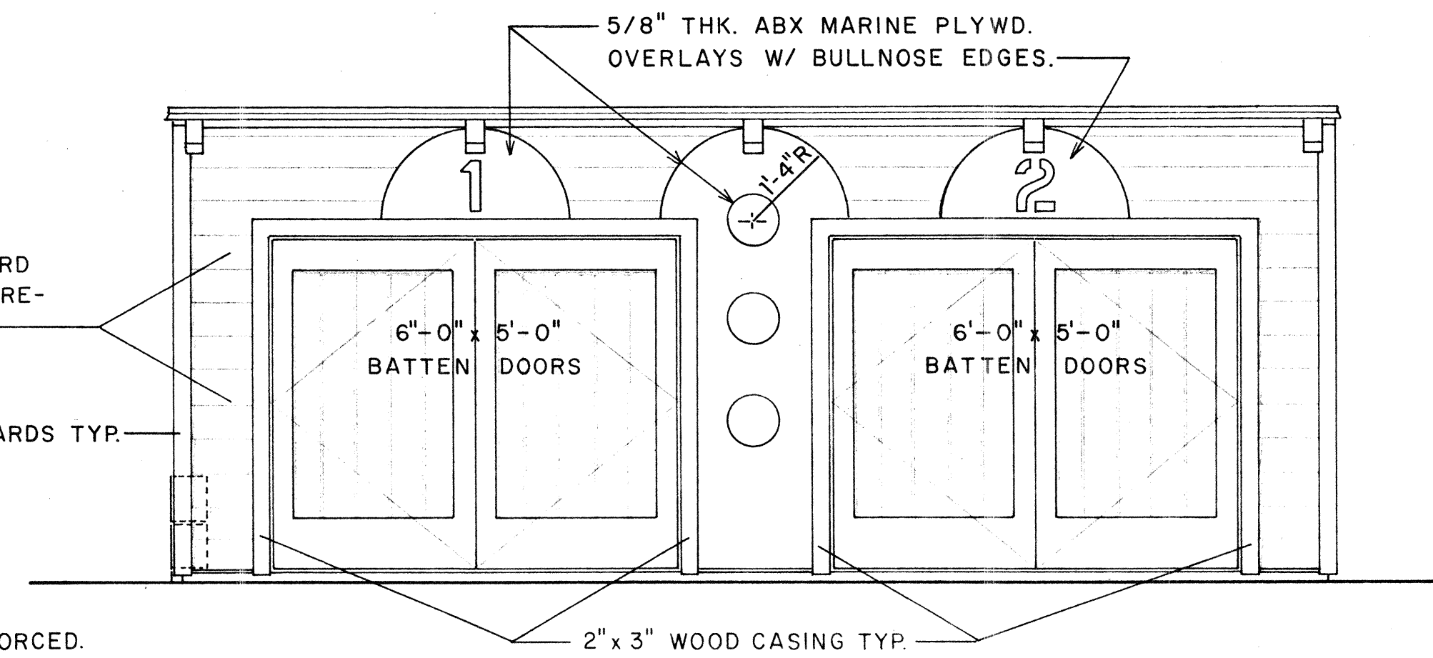
SOUTH ELEVATION OF TRICYCLE SHED
