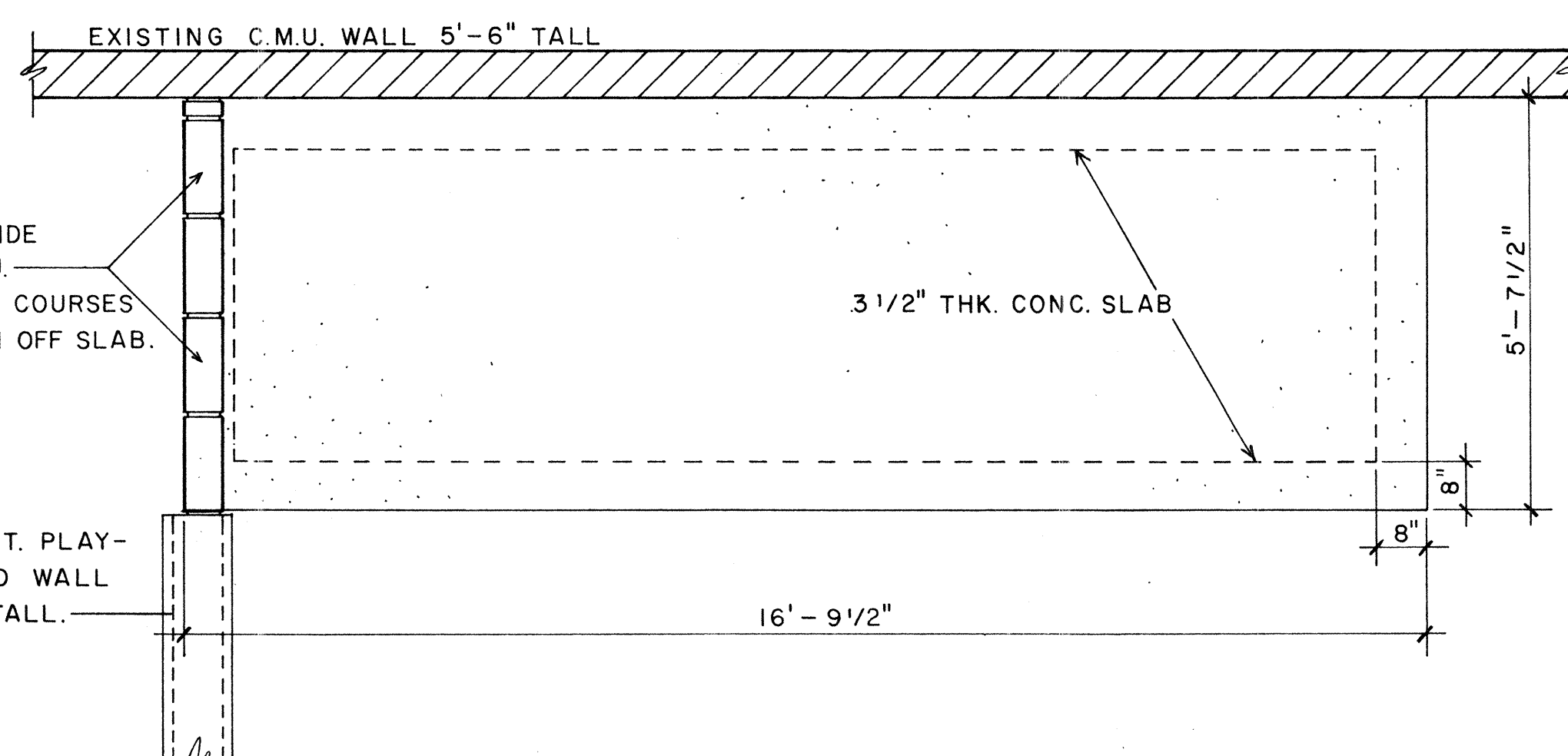
FOUNDATION PLAN
