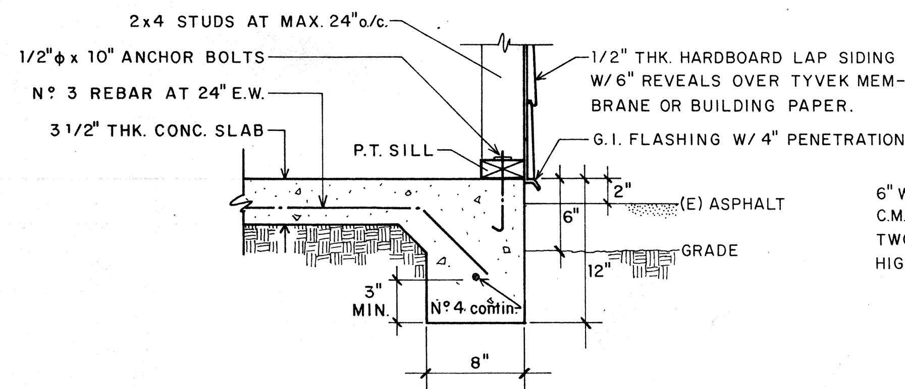
FOUNDATION DETAIL
