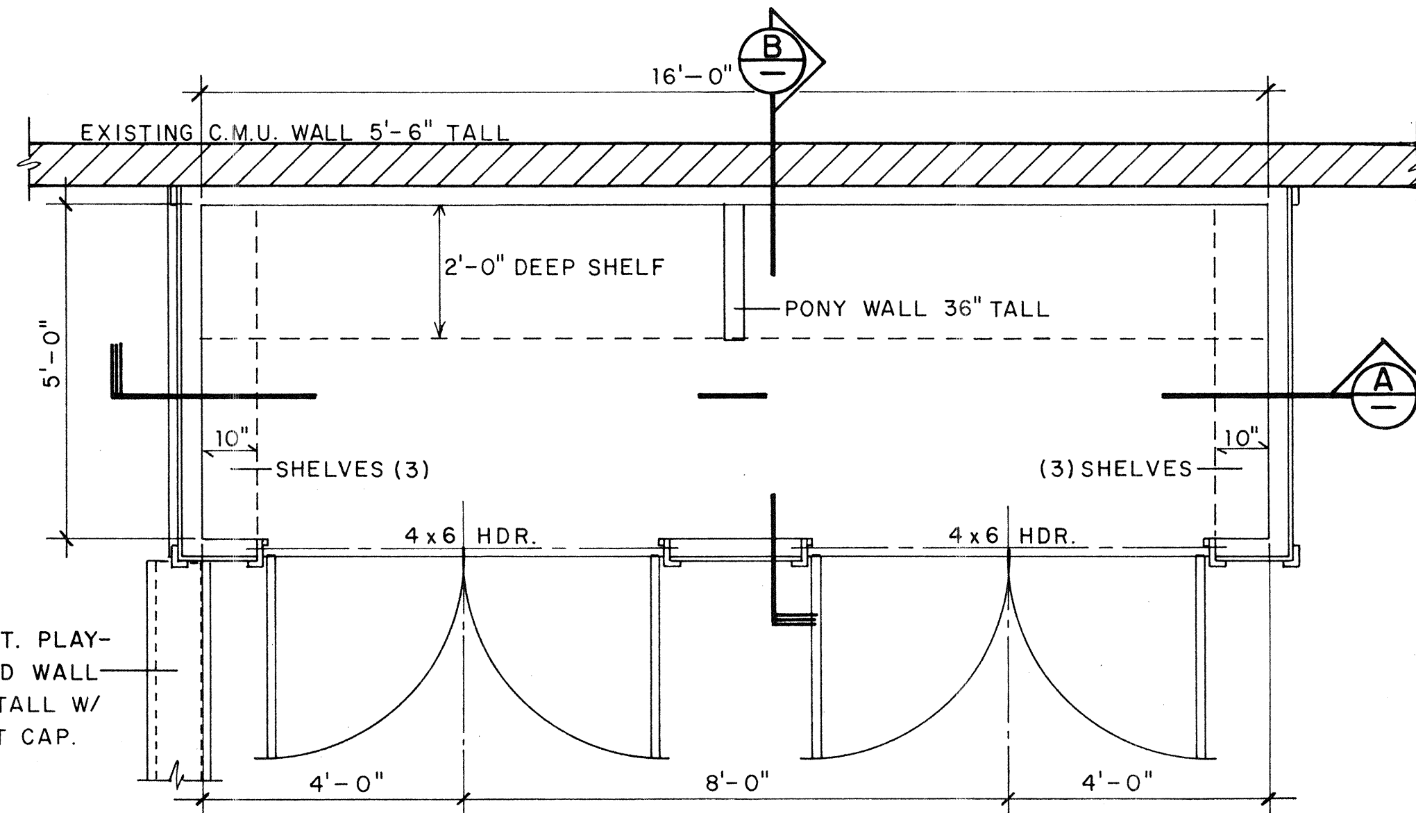
FLOOR PLAN OF TRICYCLE SHED
