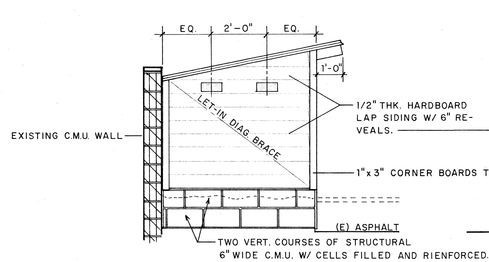
WEST SIDE ELEVATION
