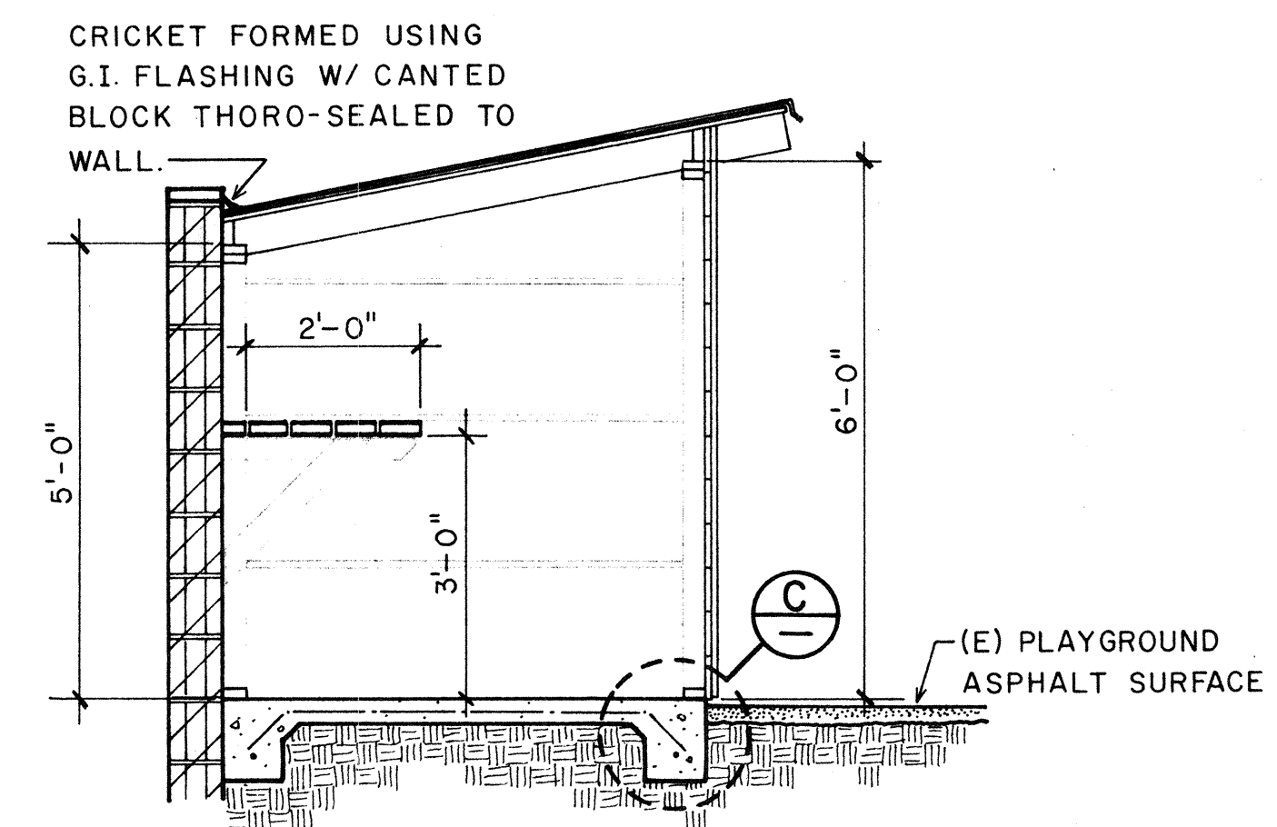
TRANSVERSE SECTION
